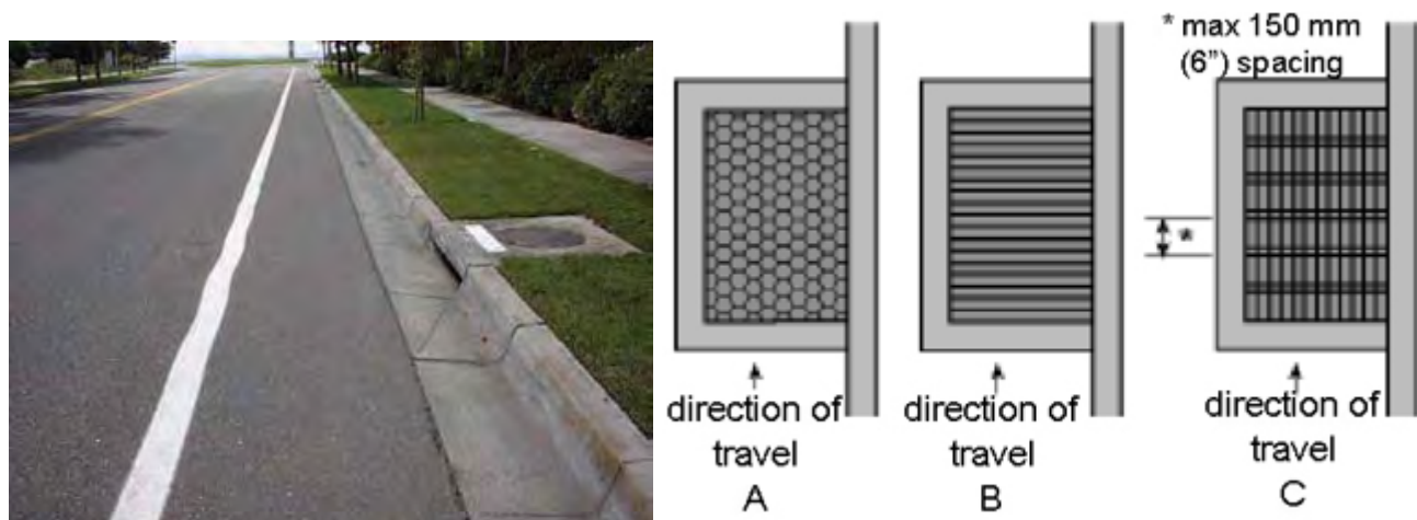
Exhibit 1. Drainage Design
